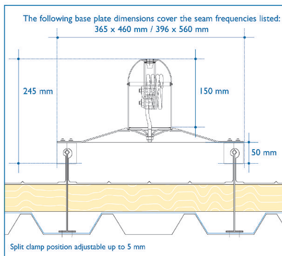
END ANCHOR
