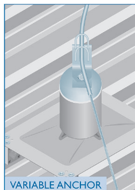
VARIABLE ANCHOR
