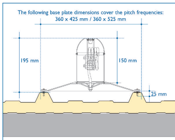
END ANCHOR
